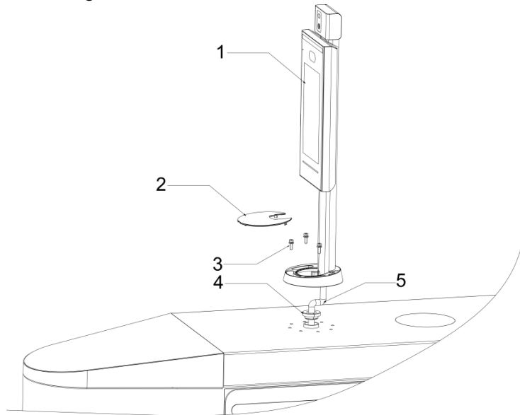
Figure 2-6 Applying silicon sealant to the terminal
