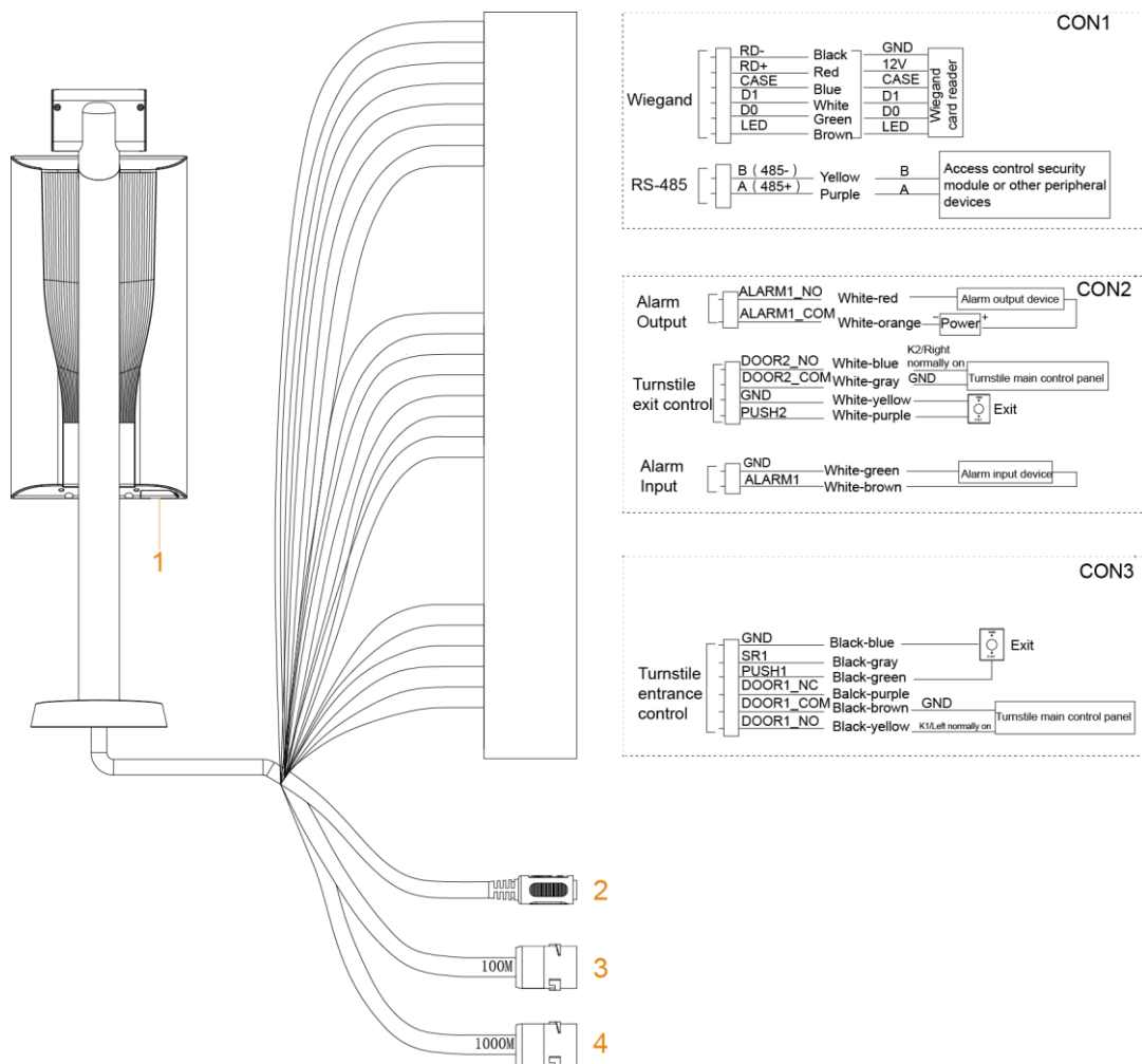
Figure 2-1 Cable connection
