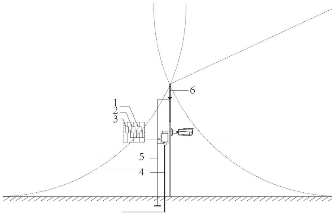
Appendix figure 1-1 Lightning protection
