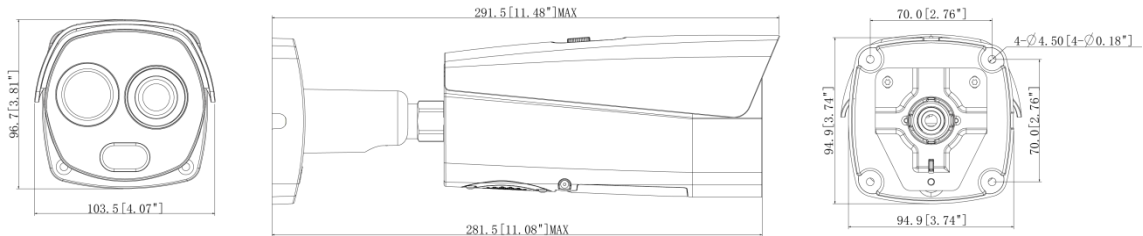
Figure 2-1 Dimension (mm [inch])
